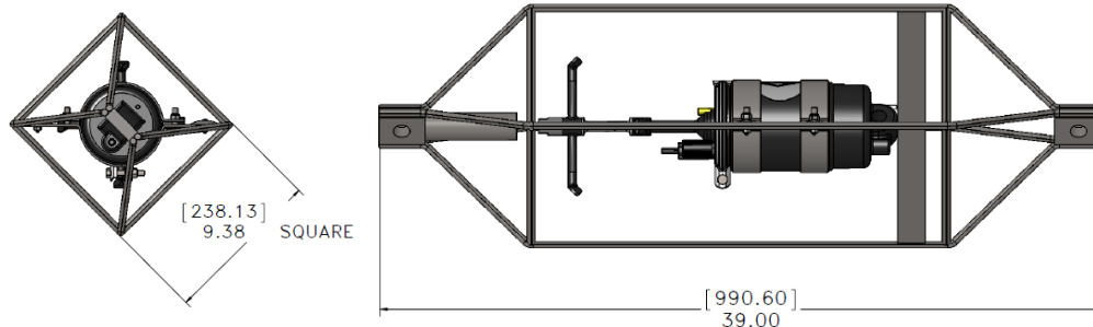
Outline Dimensions in inches [mm] are shown for the ACM-PLUS-300 with standard 5 ton Mooring Frame; contact FSI for ACM-PLUS-7000 info or further details.
